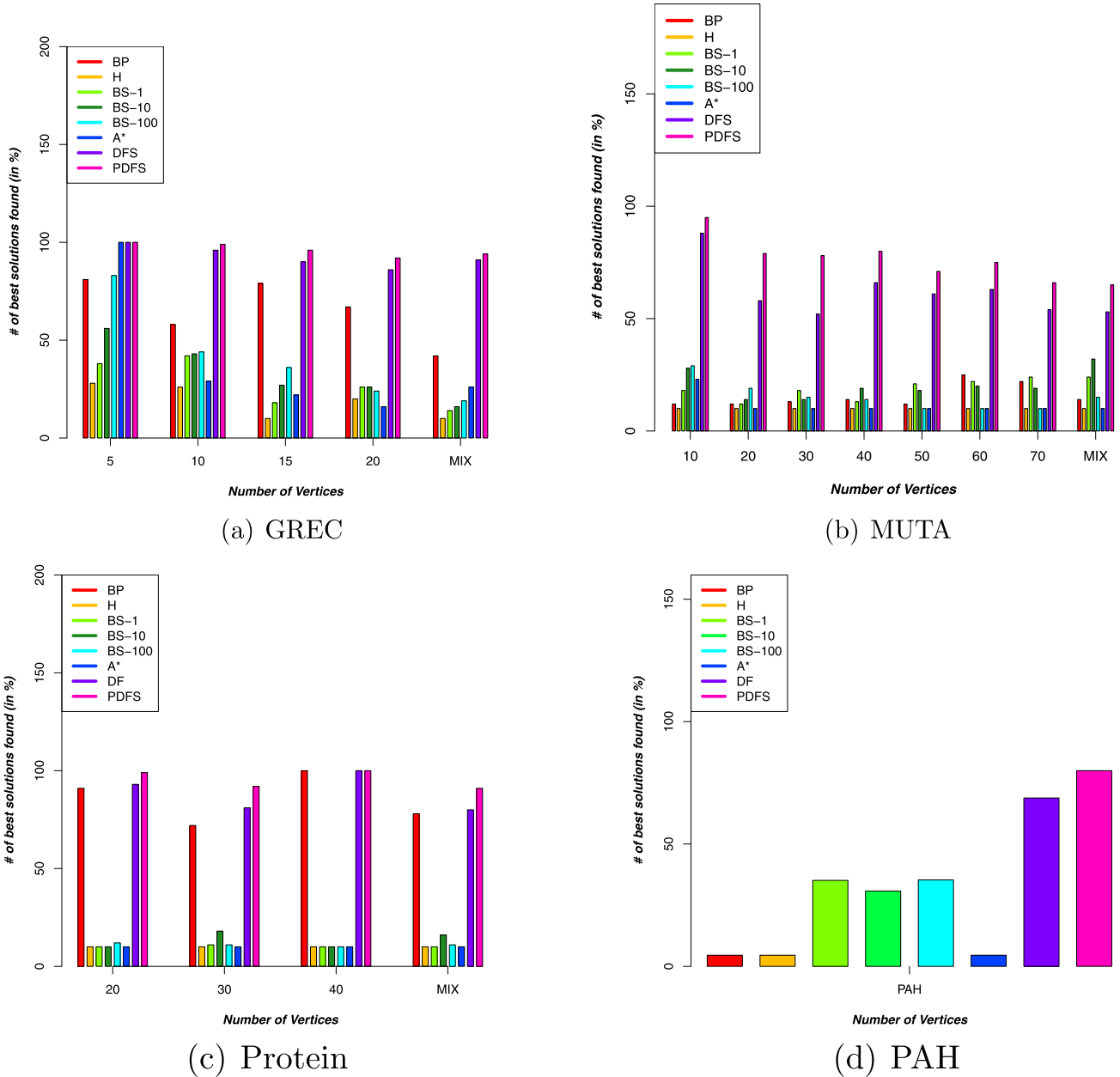
Fig. 8. Number of best found solution under small time constraint.
