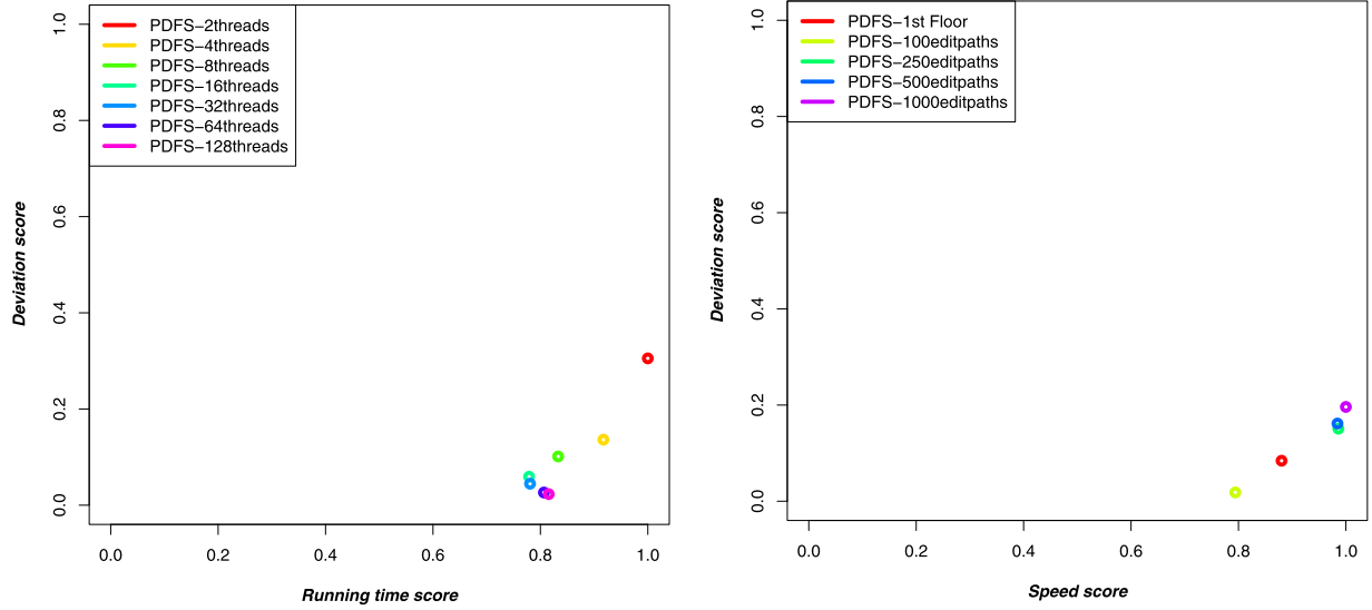
Fig. 4. Time-deviation score: left (#Threads), right (# Edit Paths).
