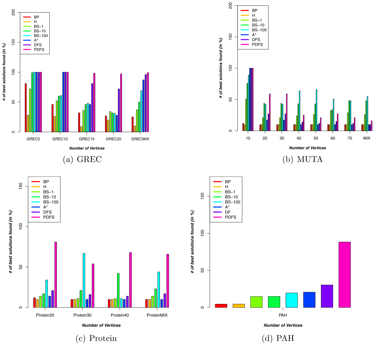
Fig. 5. Number of best found solution under big time constraint.
