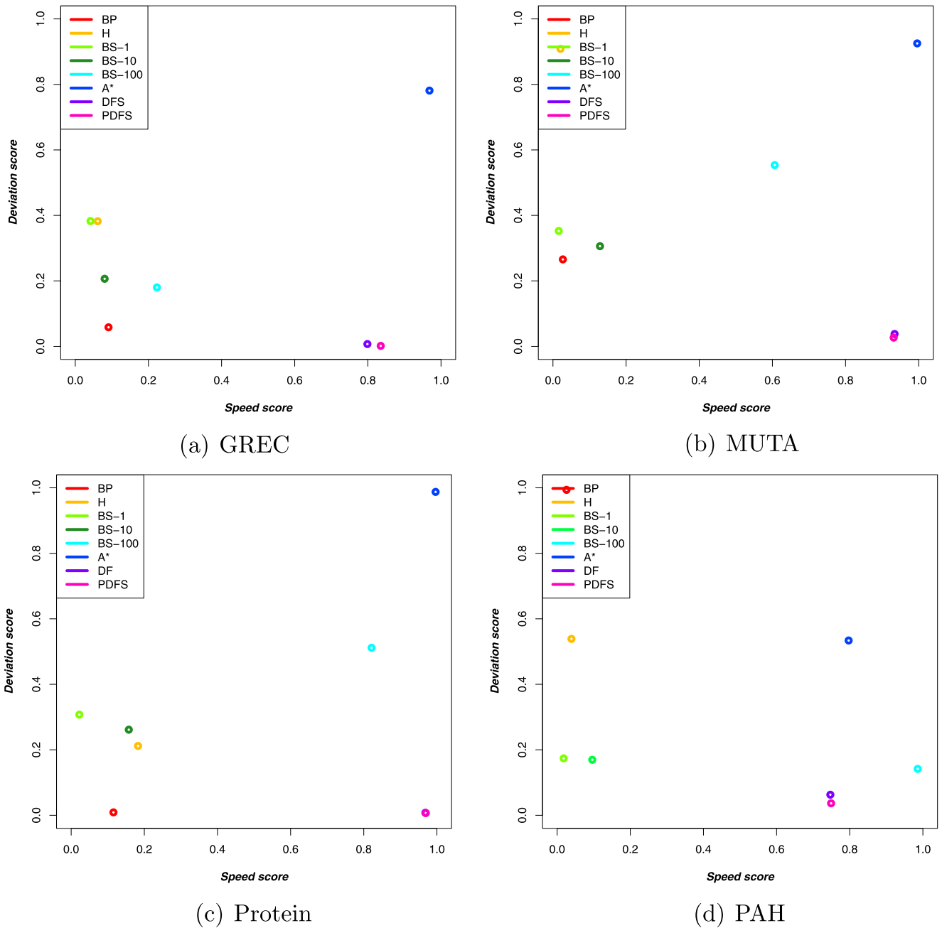
Fig. 9. Time-deviation score under small time constraint.
