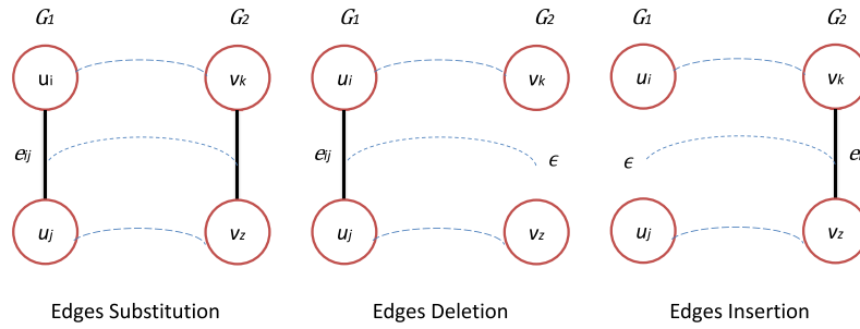
Fig. 3. Edge mappings based on their adjacent vertices and whether or not an edge between two vertices can be found.
