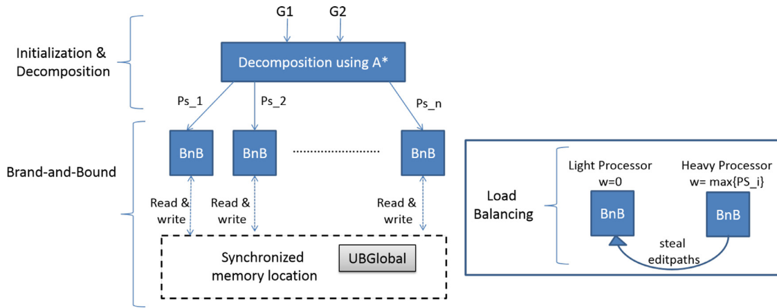
Fig. 2. The main steps of PDFS.
