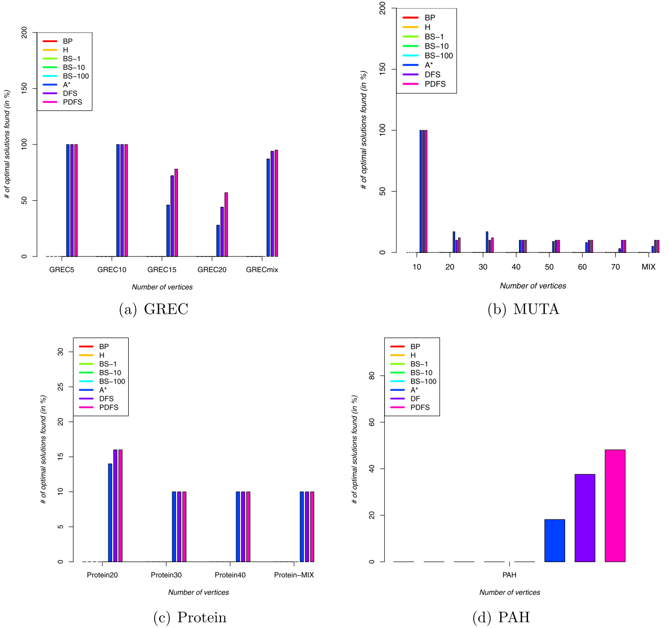
Fig. 6. Number of optimal solutions under big time constraint.
